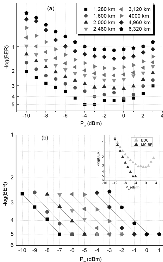
Fig. 2 BER of a nine-channel 112 Gb/s PM-4QAM transmission system without inline optical dispersion compensation as a function of launch power per channel per span. We plot various transmission reaches for (a) EDC alone for residual dispersion compensation and (b) MC-BP. Also shown in the inset is a direct comparison of the performance of the two compensation strategies after 2,000 km.
