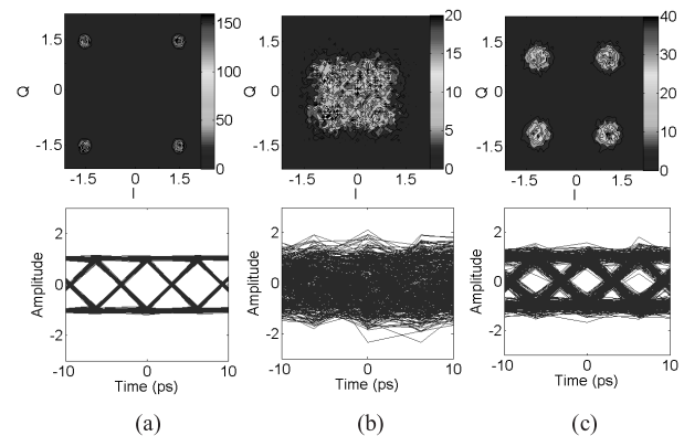
Fig. 4 Constellation maps (top) and demodulated eye diagrams (bottom) of 112 Gb/s PM-4QAM signals for a) the back-to-back signal; b) using only EDC after 6,320 km; c) using full-bandwidth back-propagation after 6,320 km.
