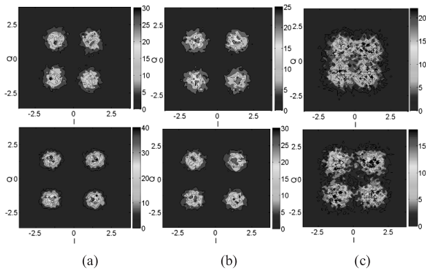
Fig. 6 Constellation diagrams after single-channel (top) and full-bandwidth (bottom) back-propagation of a nine-channel 112 Gb/s/channel PM-4QAM transmission system after 6,320 km a) for dispersion maps with 0% inline compensation; b) 50% inline compensation; c) 100% inline compensation.
