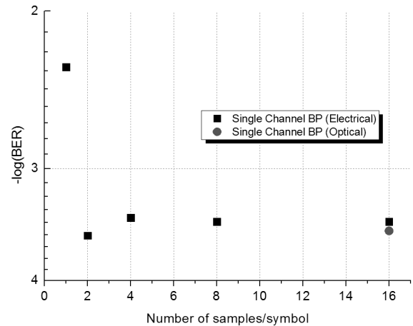
Fig. 8 BER of the electrically implemented single-channel back-propagation method as a function of the sampling rate of the ADC for a nine-channel PM-4QAM system with 0% inline dispersion compensation (and no mid-stage loss).
