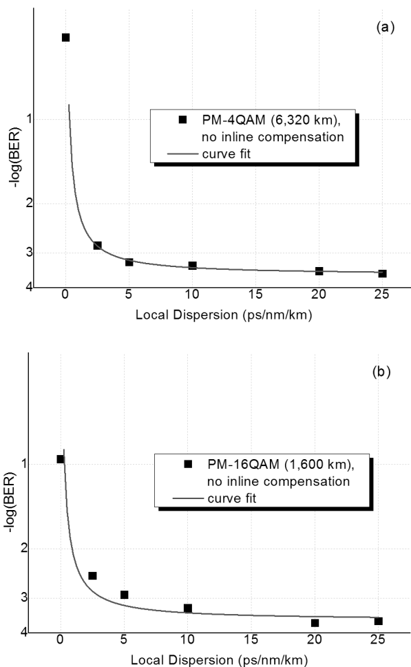
Fig. 7 BER as a function of local dispersion for a nine-channel WDM 112 Gb/s a) PM-4QAM, b) PM-16QAM, with no inline dispersion compensation (no mid-stage loss), after single-channel back-propagation. Data (symbols), Line (curve fit).
