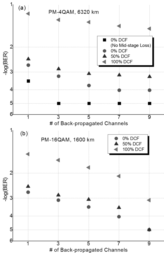
Fig. 5 Performance of back-propagation versus the number of channels included in the back-propagation computation for different dispersion maps in a nine-channel 112 Gb/s a) PM-4QAM, b) PM-16QAM system after 6,320 km and 1,600 km transmission, respectively.
