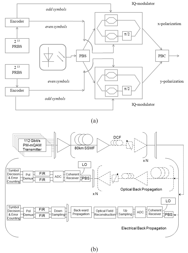
Fig. 1 Simulation setup a) PM-mQAM ( m=4,16 ) transmitter, b) WDM PM-mQAM transmission system.
