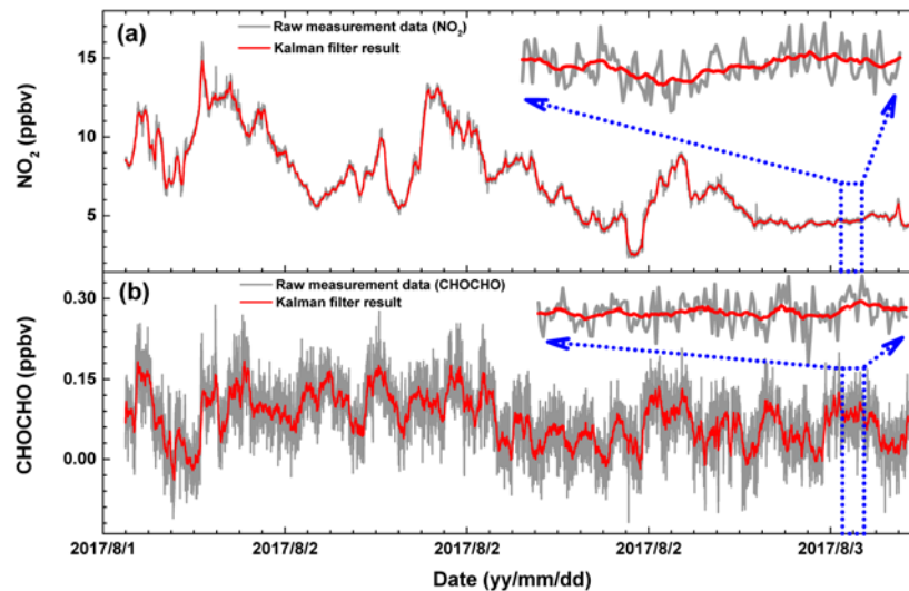
Fig. 7. Ambient air measurement of \text{NO}_2 (a) and CHOCHO (b) with the new BBCES instrument. A Kalman filter was used to improve the detection precision (red lines). The insets show a typical 1-h expanded view of the data with \rho set to 100.
