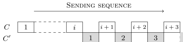
Fig. 2. Package interleaving.
