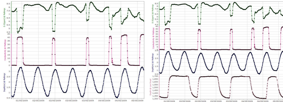
Figure 5. Multi parameter data and fusion of data from the Lee Maltings and Lee Road site
