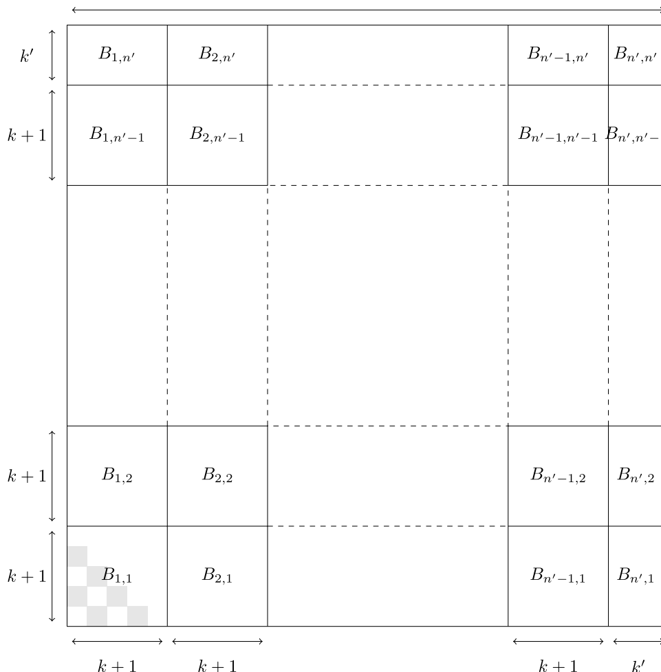
Fig. 4. Partition of the board into boxes.
