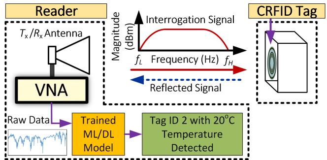
Fig. 1. Overview of an ML-assisted Chipless RFID System.
