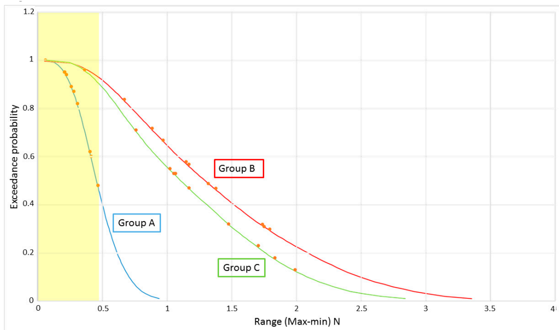
Figure 13. Exceedance plots for front line load error ranges for Groups A, B, and C.
