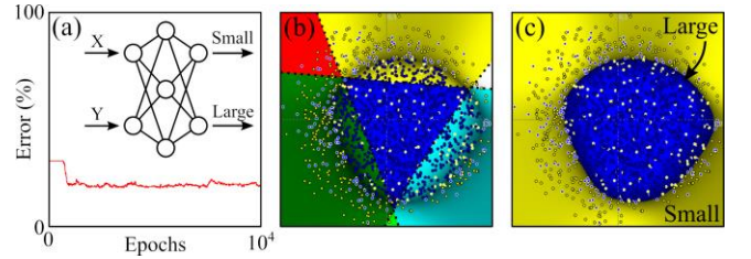
Fig. 7. Analysis of the BD spot distribution shown in Fig. 2b with a 2:3:2 neural network. (a) Training of the neural network and its schematic representation. (b) Representation of the classification (decision boundaries) carried out by the neural network. (c) Final results provided by the neural network. The blue region corresponds to large spots ( A_{BD} > 10 \mu\text{m}^2 ) and the yellow one to small spots ( A_{BD} < 10 \mu\text{m}^2 ).
