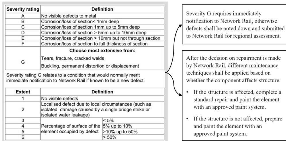
Figure 1: Severity and extent ratings for metallic elements of bridges
