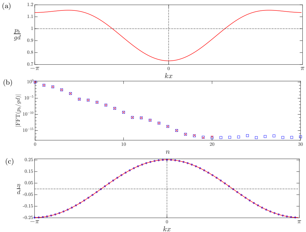
Figure 2: Same as Figure 1 for the case \omega\sqrt{d/g} = 3 , H/d = 0.5 and L/d = 2\pi .
