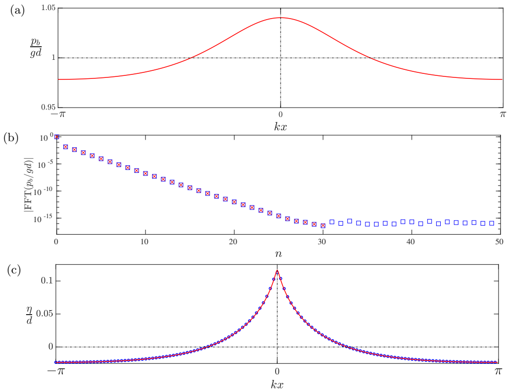
Figure 1: Example of surface recovery for \omega\sqrt{d/g} = -1.7 , H/d = 0.14 and L/d = 2\pi : (a) pressure at the bottom; (b) Fourier spectrum extracted from bottom pressure (blue squares) and fitted harmonics used for the reconstruction (red crosses); (c) recovered wave profile (red line) versus exact surface profile (blue circles).
