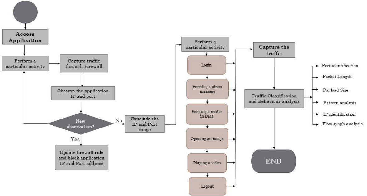
Figure 2. Analysis Framework
