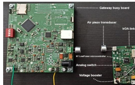
Figure 3 IMPAQT boards
