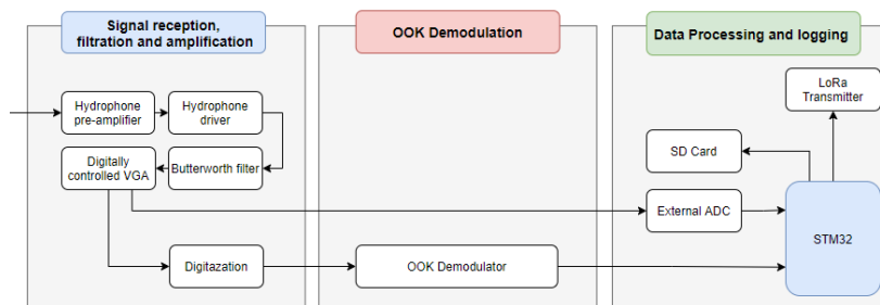
Figure 2 IMPAQT Receiver system design
