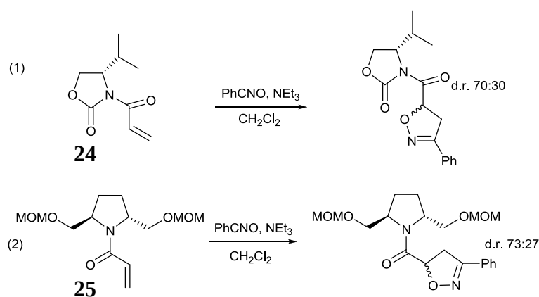
Scheme 22
