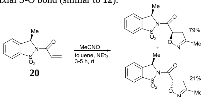
Scheme 20
