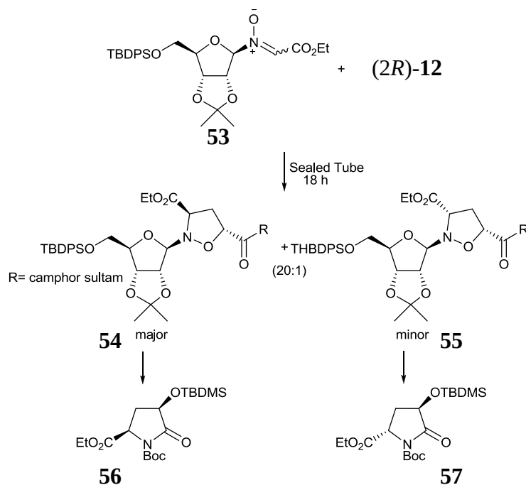
Scheme 42
