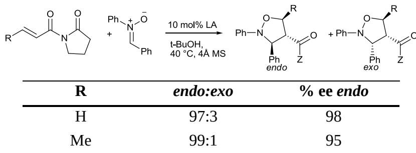
Scheme 50
