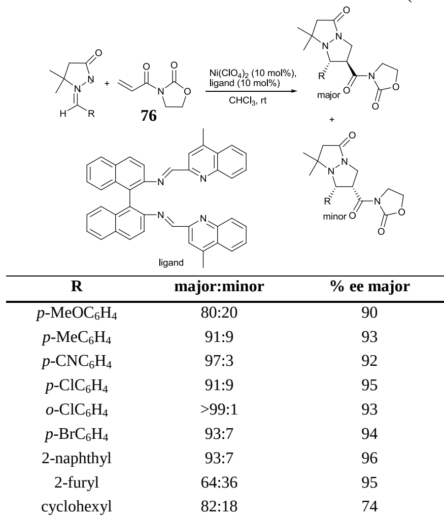
Scheme 76
