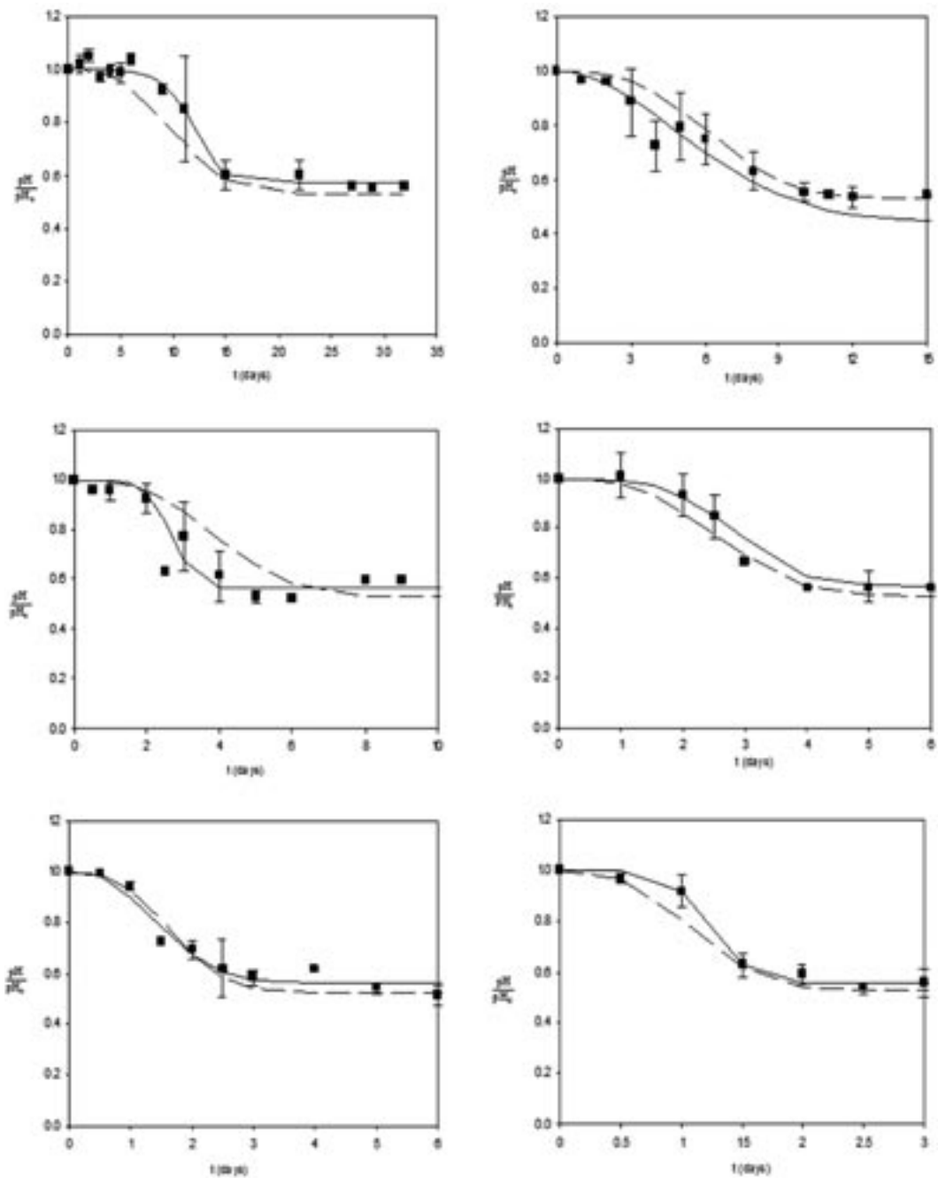
Fig. 5 - Change of the pH/pH_0 of the shredded carrots stored in air-flux system over time in a range of temperature 0^{\circ} - 20^{\circ}C . The dots represent experimental data with the standard deviation, the continuous line shows the fit of the Weibull model to the experimental data at each temperature; the break line shows the fit of the global model.
