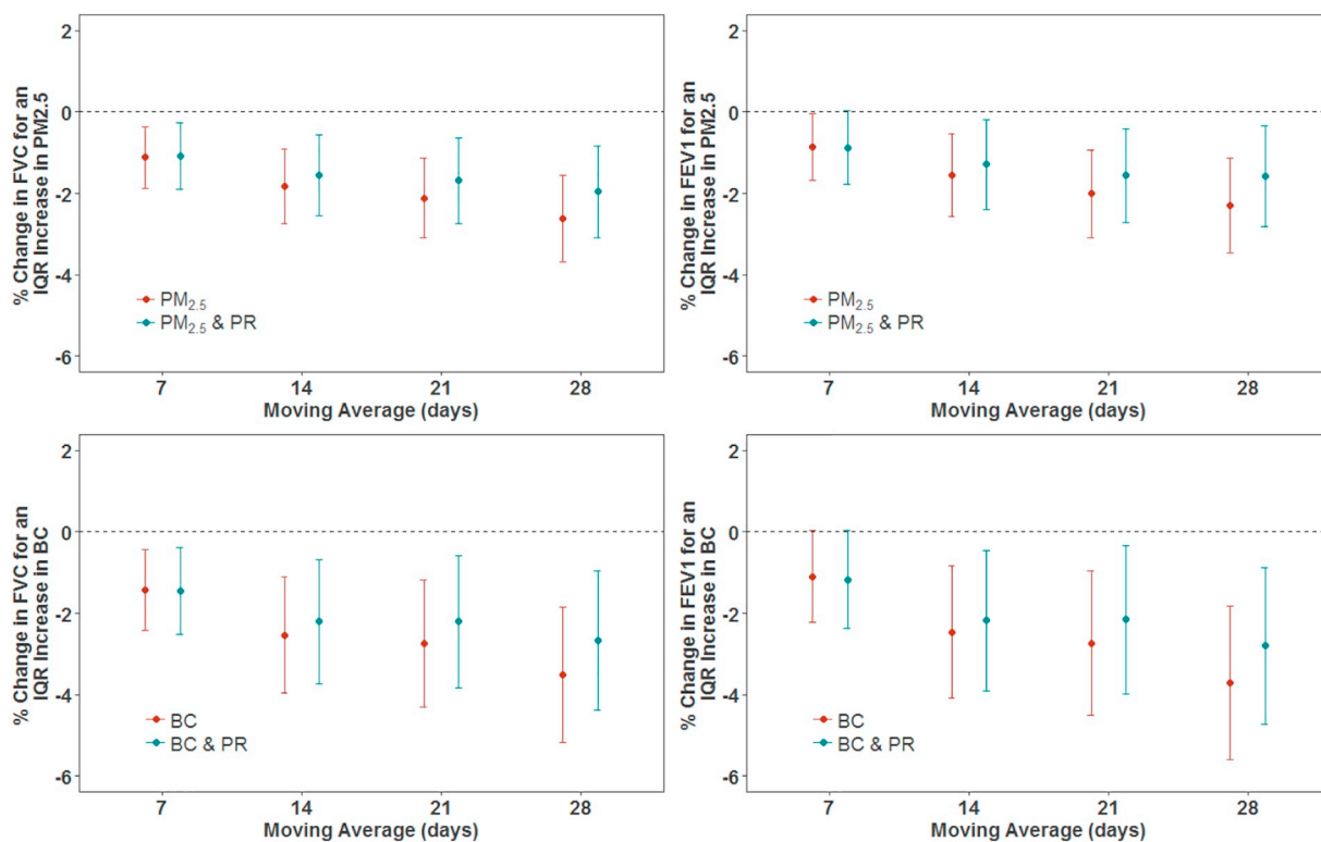
Fig. 2. Associations of particulate air pollution exposures (PM 2.5 and BC) with FVC and FEV 1 , and associations of particulate air pollution exposure with FVC and FEV 1 where the models have also included PR exposures, in a cohort of men (n = 839 subjects). All models were adjusted for age, race, height, weight, education level, smoking status, cumulative smoking, sine and cosine terms of the day of the year, day of the week, visit number, temperature, relative humidity, asthma, chronic bronchitis, emphysema, methacholine responsiveness, corticosteroids, sympathomimetics, anticholinergics. The y-axis represents the percent difference (and 95% CIs) in FVC or FEV 1 per IQR increase in PR exposure. The IQRs for PR are shown in Table 2. The IQRs for PM 2.5 mass and BC are shown in Table 2.
