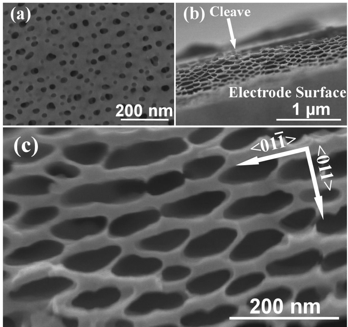
Figure 5. SEM micrographs of the (100) plane of an InP electrode anodised in 17 \text{ mol dm}^{-3} KOH at 10^\circ\text{C} at a constant potential of 0.9 V. Image (a) shows the typical electrode surface, image (b) shows where a portion of the surface was removed during sample cleavage, revealing a window on the CLO pore (100) cross section (perpendicular to pore growth direction), which is shown at a higher magnification in image (c). The inset in (c) shows the crystallographic orientation of all of the images.
