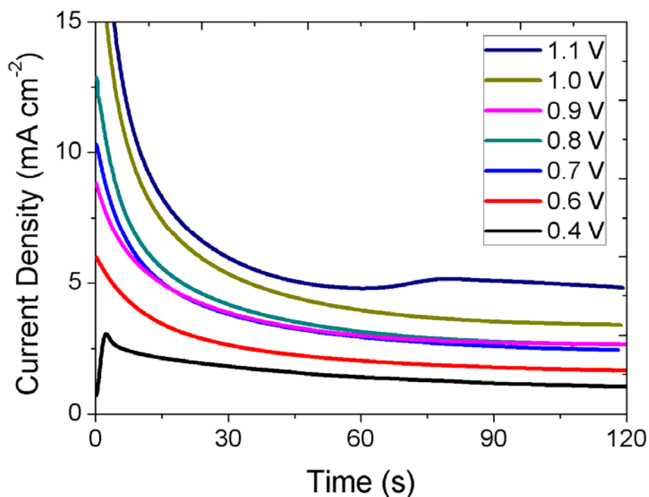
Figure 3. A series of current-time plots of InP electrodes anodised at constant potentials in 17 \text{ mol dm}^{-3} KOH at 10^\circ\text{C} . The anodisation potentials range from 0.4 to 1.1 V.
