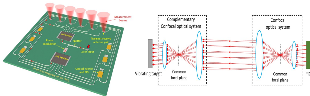
Fig. 1. (a) Schematic show of the external confocal optical system, the six-beam LDV on an SOI-based photonic integrate circuit (PIC). (b) Schematic show of the system used in the de-speckle experiments. The dimensions of the lenses in the drawing are exaggerated to make the design easier to understand.
