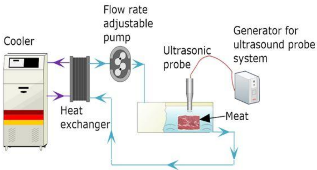
Figure 2. Schematic diagram of experimental set-up. The system used was composed of a refrigerated circulator (cooler), through which glycol coolant ( -0.5\text{ }^{\circ}\text{C} ) was circulated using a heat exchanger and a pump, The meat sample was fixed horizontally onto a basket in a tank filled with 15% brine solution. Ultrasound (US) with a frequency of 20 kHz was irradiated onto the sample for 60 minutes by using an ultrasonic processor.
