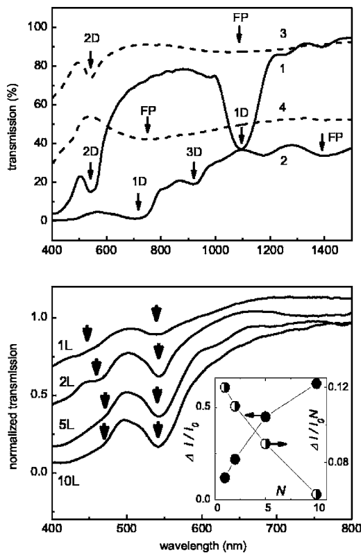
FIG. 1. (a) s -polarized transmission spectra of 1L (dash) and 10L (solid) LB films at \theta=0^\circ (curves 1 and 3) and 70^\circ (curves 2 and 4). The arrows indicating the minima are labeled according to their origin. (b) Normalized transmission spectra of LB multilayers. The curves are shifted for clarity. The arrows are to guide the eye. Inset: relative attenuation \Delta I/I_0 at 545 nm minimum and the specific relative attenuation \Delta I/I_0 per layer as the function of the number of layers N .
