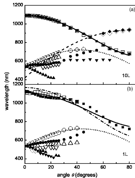
FIG. 4. (a) Dispersion of transmission minima of 10L film in s (solid symbols) and p (open symbols) polarizations. The solid and dashed lines denote Bragg fits to the diffraction at 1D stack of LB monolayers and 3D diffraction, respectively. The dotted line is a fit to diffraction of a 2D grating. (b) The same for 1L film. The solid and dashed lines denote Bragg fits to the diffraction at 1D stack of LB monolayers using two and one free parameters, respectively.
