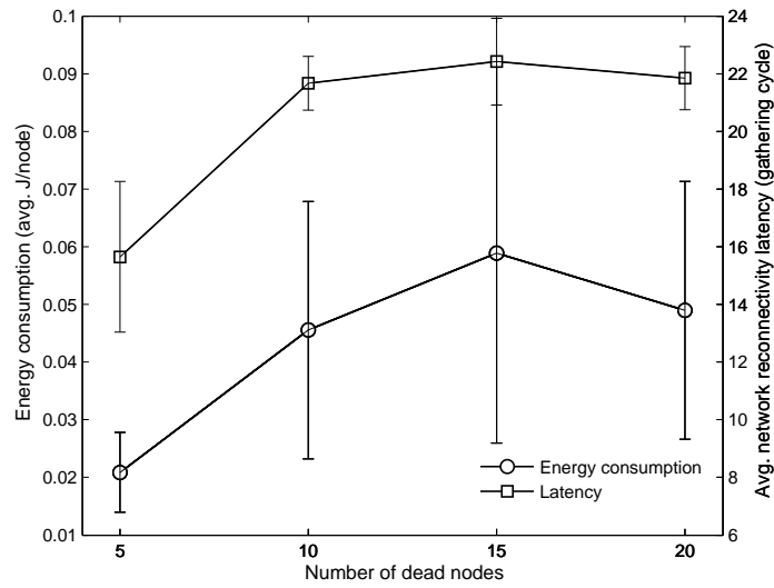
Figure 23: Energy consumption and latency of ER-MAC for network reactivity when some nodes die simultaneously
