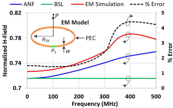
Fig. 2. EM model (inset) and normalized H-Field and % error vs frequency. Note that % error = 100 \times (H_{EM} - H_{ANF})/H_{EM} , where H_{EM} and H_{ANF} are the normalized H-fields associated with the EM and ANF methods respectively.
