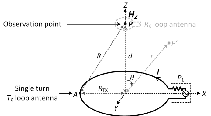
Fig. 1. Near-Field inductive coupling between two loops in free-space, denoted T_X and R_X .
