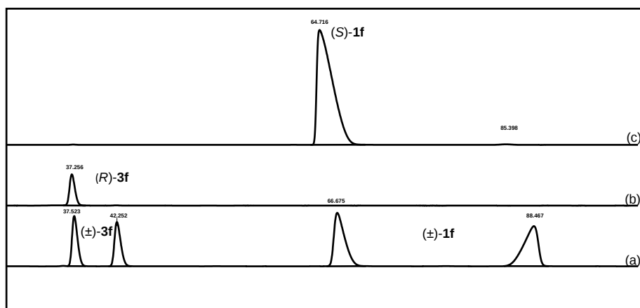
Figure 2: An overlay of HPLC traces of (a) A racemic mixture of ethyl 3-(3-methylphenyl)butanoic acid (±)- 1f and ethyl 3-(3-methylphenyl)butanoate (±)- 3f . (b) Enantiopure ethyl 3-(3-methylphenyl)butanoate ( R )- 3f and (c) Enantiopure 3-(3-methylphenyl)butanoic acid ( S )- 1f . See Table 7 for chiral HPLC conditions.
