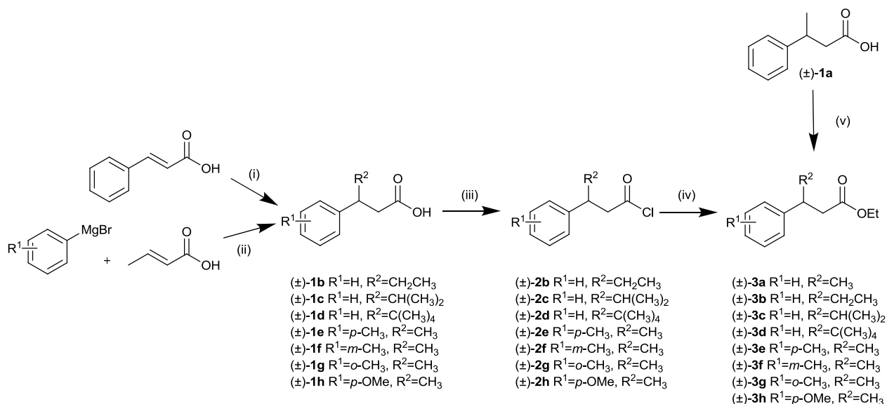
Scheme 1. Synthesis of ethyl 3-aryl alkananoate (±)- 3a-h . Reagents: (i) R²MgX, Et₂O, (±)- 1b-d ; (ii) Et₂O, (±)- 1e-h ; (iii) SOCl₂; (iv) Et₃N, EtOH, CH₂Cl₂; (v) EtOH, cat. H₂SO₄, (±)- 1a .
