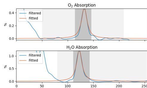
Figure 3. Gas absorption signals
