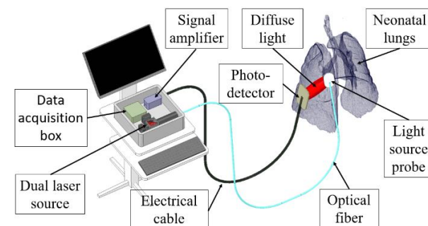
Figure 1. Schematic drawing of the lung analyzer system
