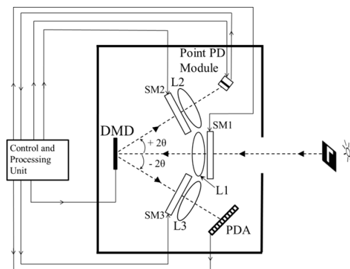
Fig. 1. CAOS smart camera design for sensing and tracking diverse spatial and spectral targets.
