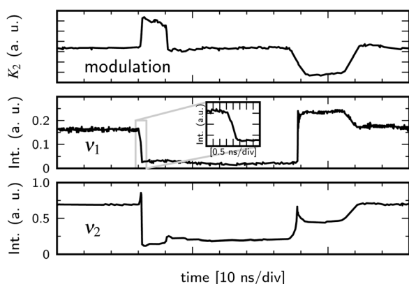
FIG. 4. The intensity times traces of the modulated injection K_2 (top), and the modes v_1 (middle) and v_2 (bottom) for detunings as in Fig. 3. The modulation range is indicated by the arrows in Fig. 3. The inset shows the falling edge of mode v_1 switching from on to off states, where the 90:10 switching time is < 500 ps.
