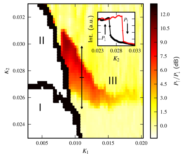
FIG. 3. (Color online) Partition of the K_1 - K_2 plane for \Delta\nu_1=-8 GHz and \Delta\nu_2=-18 GHz into three regions: I contains no locked states; II comprises of one locked state and one unlocked state; and region III consists of only locked states. The inset shows hysteresis of the linear power in mode 1 at K_1=0.01 for up ( P_1 ) and down ( P_1 ) sweep in K_2 as indicated by the arrows in the main panel. The color of region III represents the contrast ratio P_1 to P_1 (in dB) between these up and down sweeps, where the dark shading indicates a large contrast of optical power in mode one.
