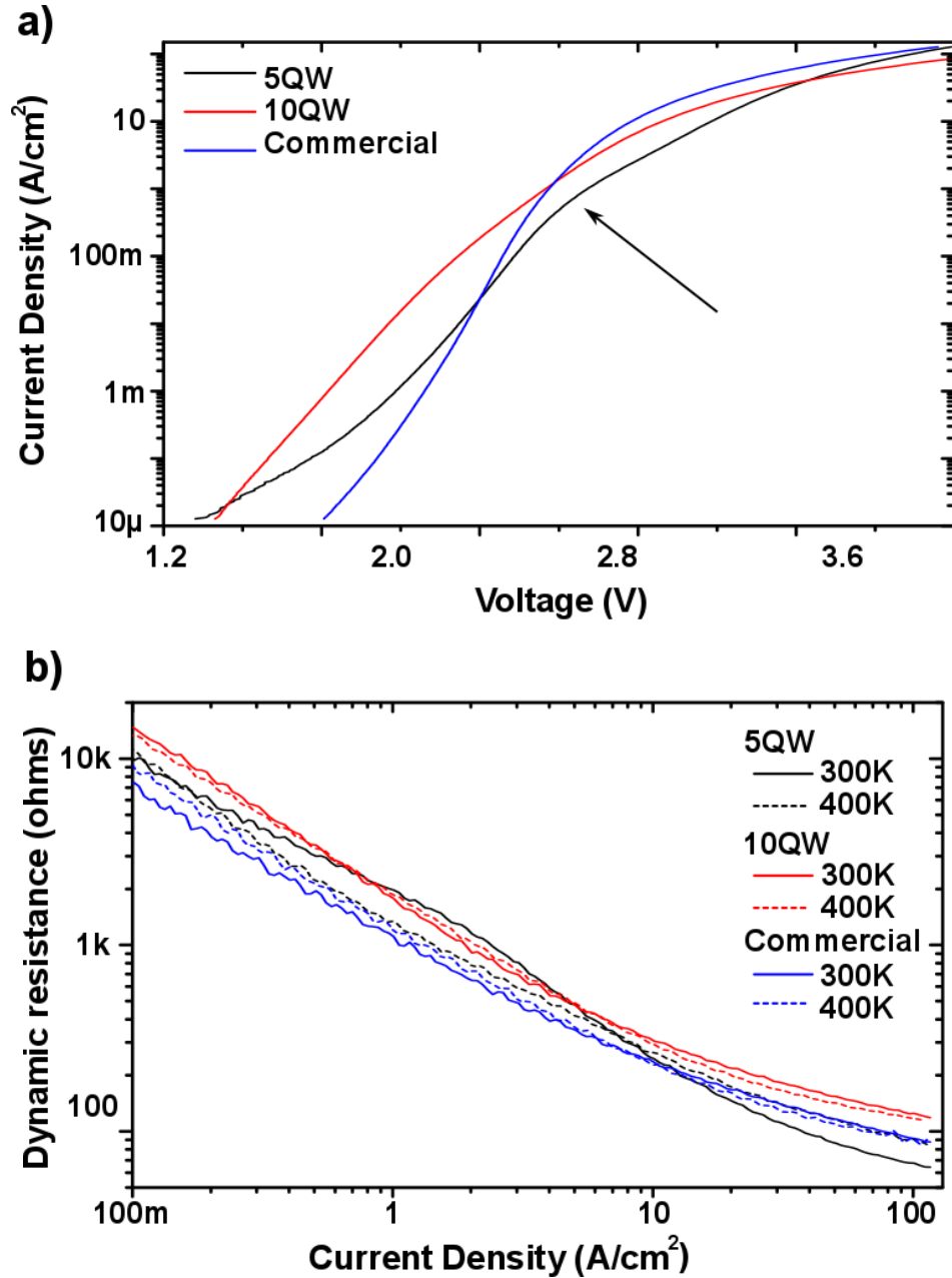
Figure 5.3: a) Semi-log scale current density - voltage (J-V) curve at 300 K illustrating the different exponential rise of current for each sample. The arrow highlights a change in character for the 5QW sample. b) Semi-log scale dynamic resistance versus current at 300 K (continuous lines) and at 400 K (dotted lines).
