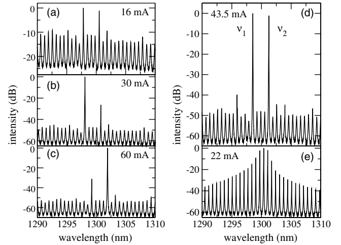
FIG. 3. (a) Below threshold spectrum of the two-color device of Fig. 2. (b) Lasing spectrum at 30 mA. (c) Lasing spectrum at 60 mA. (d) Two-color lasing spectrum at 43.5 mA. (e) Above threshold spectrum of a plain Fabry-Pérot device fabricated on the same bar.
