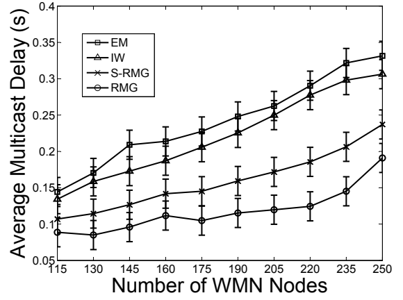
Fig. 12. The average delays when the WMN size increases from 115 to 250.
