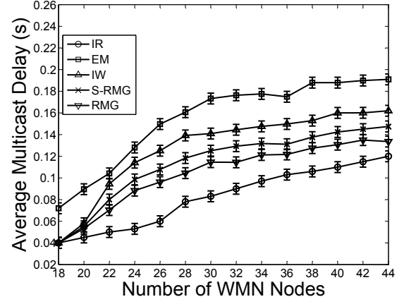
Fig. 7. The average delay performance when the WMN size in Fig. 6 increases from 18 to 44.
