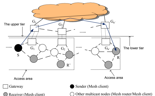
Fig. 1. An example of the two-tier integrated architecture .
