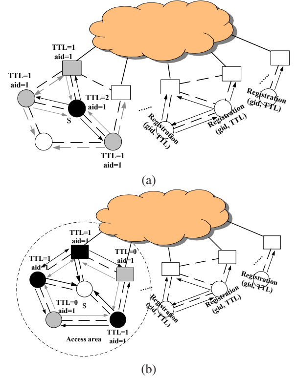
Fig. 3. An example of the access area construction . Square nodes represent gateways. Circle nodes represent mesh routers/mesh clients. Black nodes and grey nodes are the senders and the receivers of AREA_CONSTRUCTION respectively.
