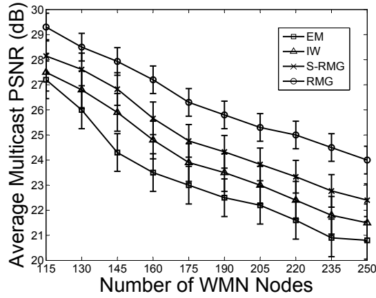
Fig. 15. The average PSNR performance when the WMN size increases from 115 to 250.
