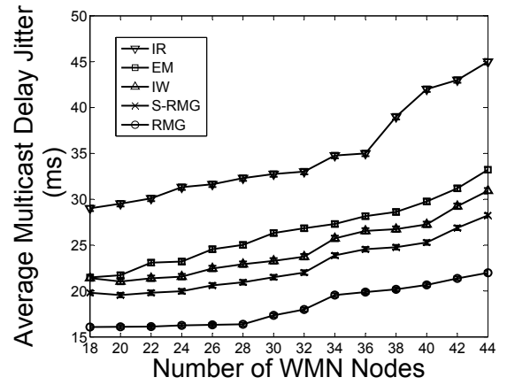
Fig. 9. The average delay jitter performance when the WMN size in Fig. 6 increases from 18 to 44.
