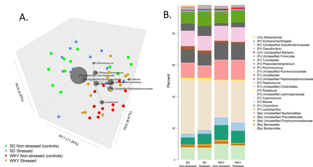
Figure 2. Caecal Microbiota. (A) PCoA biplot of unweighted Unifrac phylogenetic distances of the caecal communities in SD and WKY rats. Grey circles show the nine most relatively abundant genera where diameter is proportional to the mean relative abundance across all samples, with distance from origin (X0, Y0, Z0) indicating contribution to the variation along the principal components. (B) Bar plot of the mean relative abundance of the 25 most prevalent bacterial genera across all samples. Codes in parentheses indicate phylum; Ve = Verrucomicrobia, Pr = Proteobacteria, Fi = Firmicutes, Ba = Bacteroidetes, Un = Unclassified.
