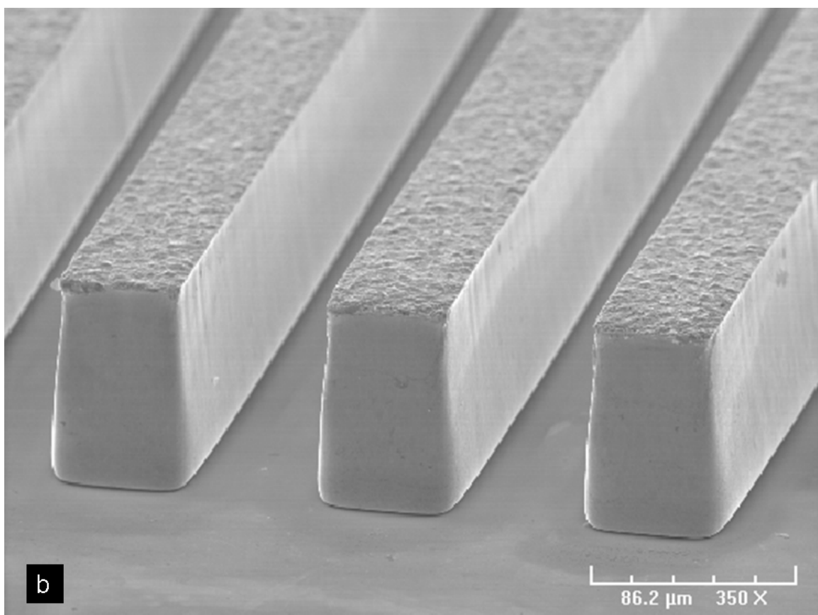
Fig. 2. (a) Electroplated Ni microstructure on Si wafer (b) 60 μm Ni lines and 60 μm gap.
