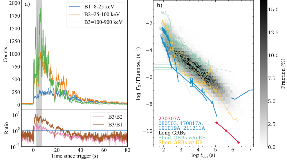
Fig. 1 The high energy properties of GRB 230307A. Panel a shows the light curve of the GRB at 64 ms time resolution with the Fermi /GBM. The shaded region indicates the region where saturation may be an issue. The burst begins very hard, with the count rate dominated by photons in the hardest (100-900 keV) band, but rapidly softens, with the count rate in the hard band being progressively overtaken by softer bands (e.g. 8-25 keV and 25-100 keV) beyond \sim 20 s. This strong hard-to-soft evolution is reminiscent of GRB 211211A [20] and is caused by the motion of two spectral breaks through the \gamma -ray regime (see Methods). Panel b shows the X-ray light curves of GRBs from the Swift X-ray telescope. These have been divided by the prompt fluence of the burst, which broadly scales with the X-ray light curve luminosity, resulting in a modest spread of afterglows. The greyscale background represents the ensemble of long GRBs. GRB 230307A is an extreme outlier of the > 1000 Swift -GRBs, with an extremely faint afterglow for the brightness of its prompt emission. Other merger GRBs from long bursts occupy a similar region of parameter space. This suggests the prompt to afterglow fluence could be a valuable tool in distinguishing long GRBs from mergers and those from supernovae.
