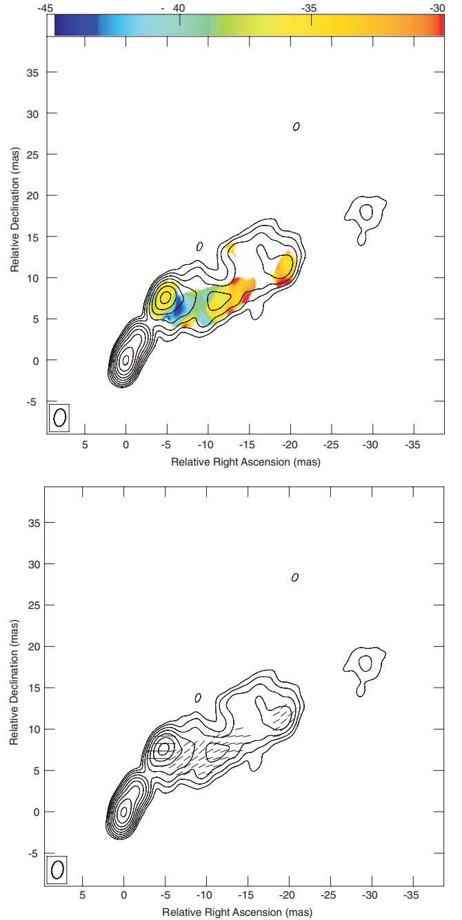
Figure 8. Top panel: RM map superimposed on 5-GHz total intensity contours of 3C 380. Bottom panel: MVPA sticks of constant length superimposed on 5-GHz total intensity contours of 3C 380. Absence of RM values and subsequently the MVPAs at the core is due to lack of 1.6-GHz polarization there. Peak flux density is 745 \text{ mJy beam}^{-1} . First contour is 2 \text{ mJy beam}^{-1} . Contour intervals at -1, 1, 2, 4 \dots times the first contour. The beam size in both images is 2.14 \times 1.37 \text{ mas} .
