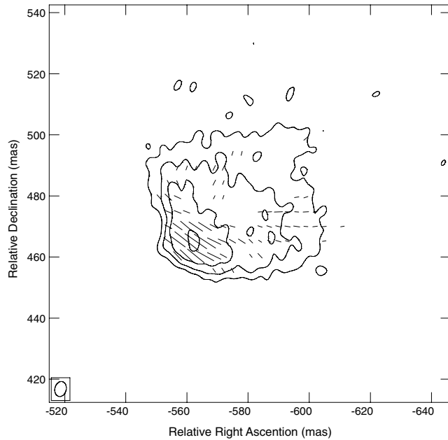
Figure 12. Faraday derotated MVPA sticks superimposed on 1.6-GHz total intensity contours of knot K1 in 3C 380. Peak flux density is 148 \text{ mJy beam}^{-1} . First contour is 2 \text{ mJy beam}^{-1} . Contour intervals at -1, 1, 2, 4 \dots times the first contour. The beam size is 5.0 \times 3.7 \text{ mas} .
